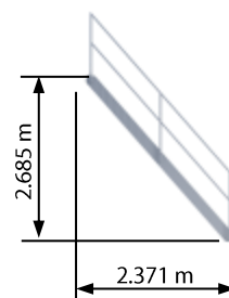
AIR-Step Treppe steil Art. 4960S
